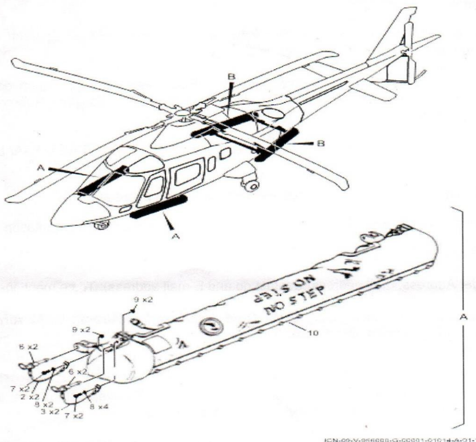
Figure: Emergency Float Assy
